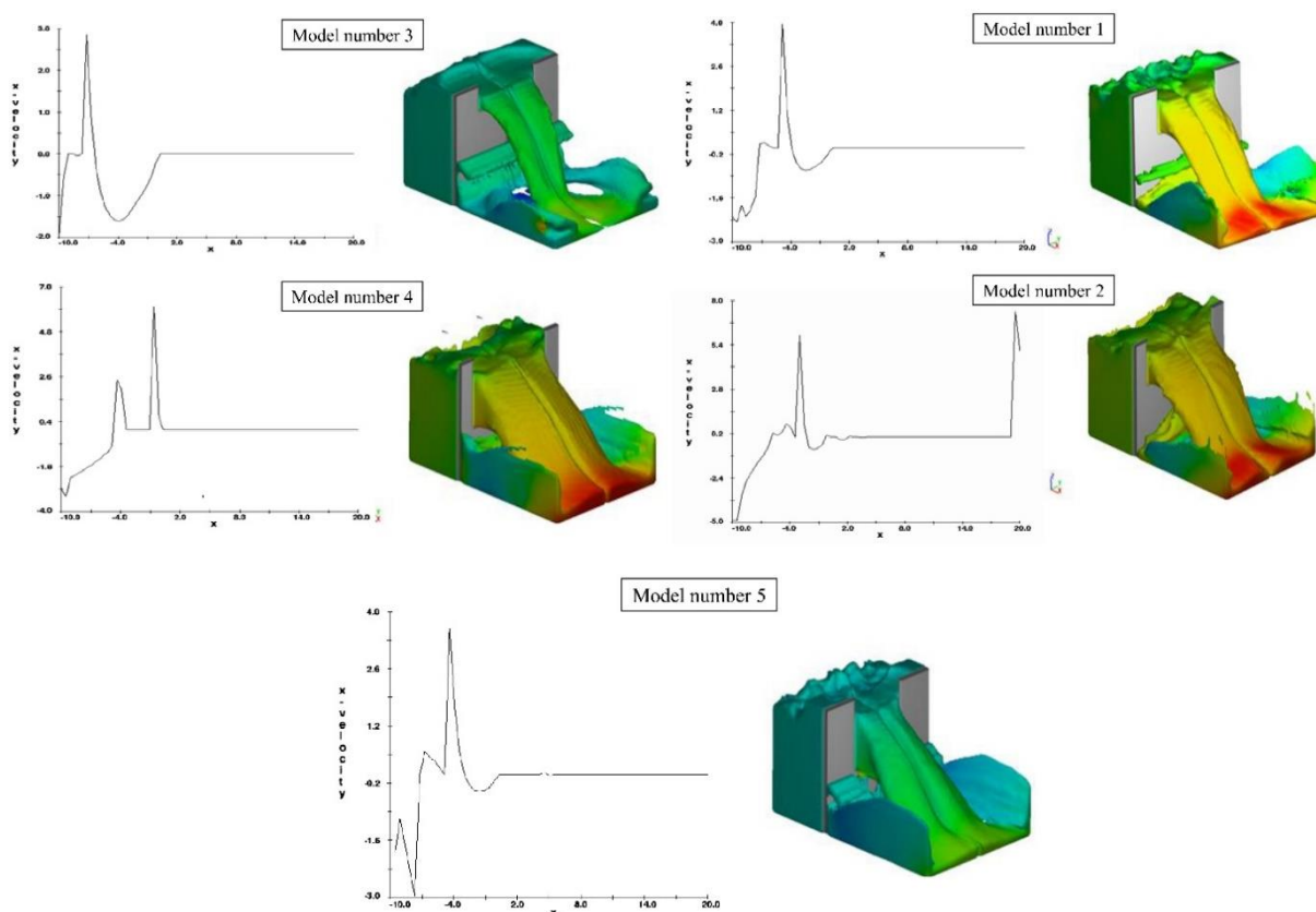
Figure 5: Flow distribution in all types of rectangular weirs
